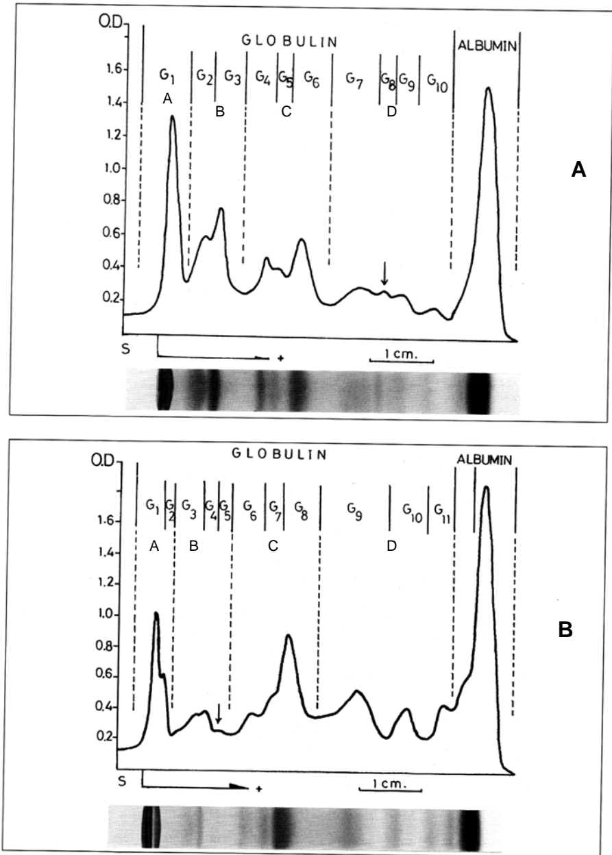
Fig. 1. Electropherograms (gel photographs) showing the electrophoretic separation of the bloodserum proteins of adult female specimens of the Lacerta laevis complex from northern Cyprus (A) and southern Turkey (B), together with their densitometric tracing curves. Designations G 1 to G 11 indicate the globulin zone fractions or fraction groups.
