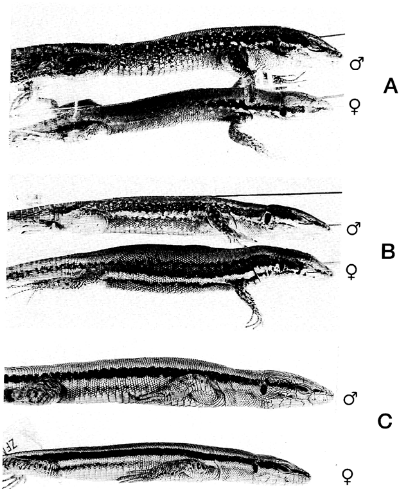
Fig. 2. Lateral view of various specimens of the Lacerta laevis complex from different localities: A: Turkey ( L. l. laevis ), ♂ ZDEU-111/1977-4, Sebil, Tarsus-Mersin and ♀ ZDEU-88/1968-7, Mezitli-Mersin; B: Cyprus ( L. troodica ), ♂ ZDEU-136/1993-3, Girne and ♀ ZDEU-93/1991-10, Çatalköy-Girne; C: Syria/Anti-Lebanon ( L. l. kulzeri ), ♂ ZFMK-57942, Rankus and ♀ ZFMK-57943, Rankus.
